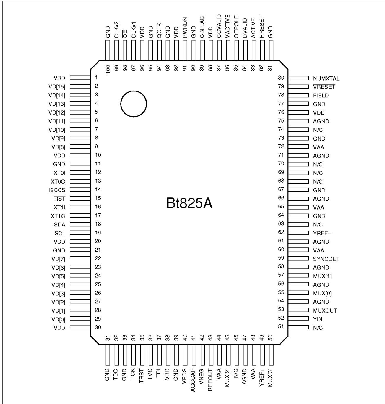
Figure 3. Bt825A Pinout
