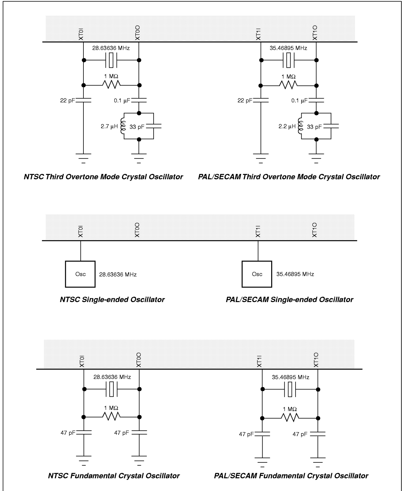
Figure 28. Clock Options
