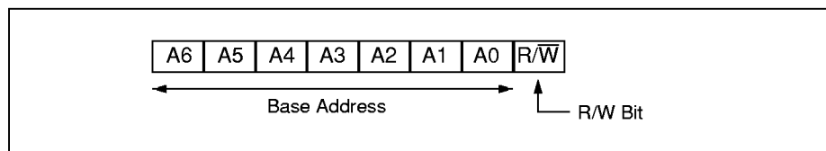
Figure 38. I 2 C Slave Address Configuration
