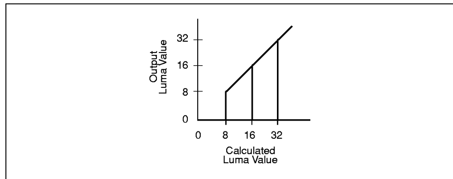
Figure 25. Coring Map
