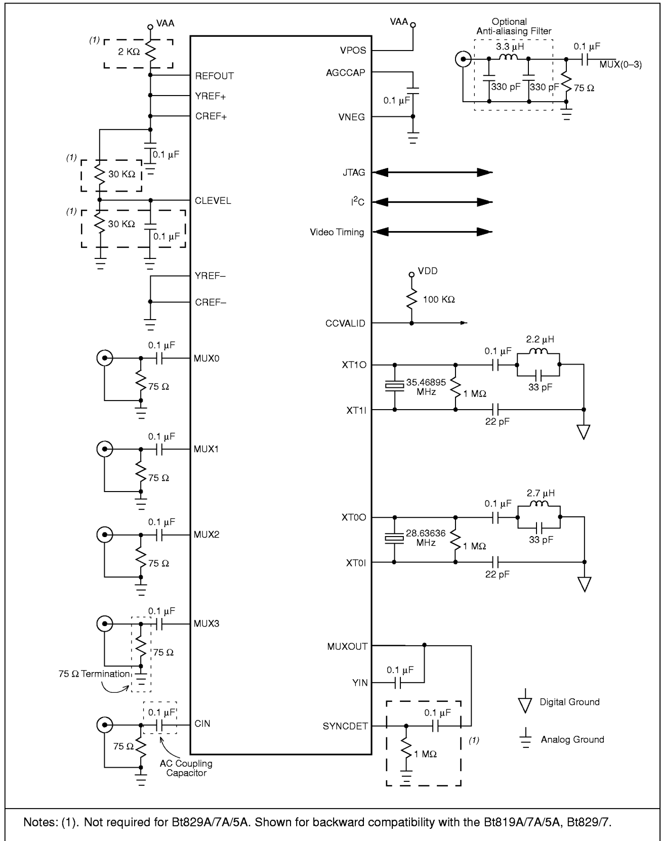
Figure 26. Bt829A Typical External Circuitry for Backward Compatibility with Bt819A/7A/5A
