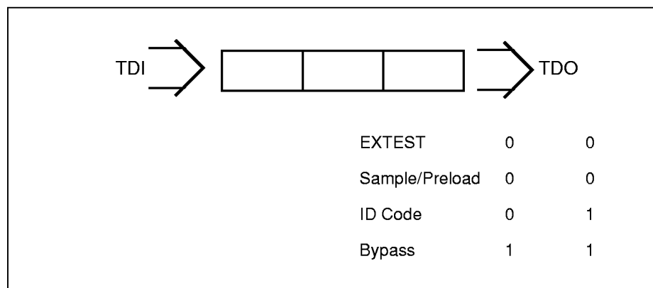
Figure 40. Instruction Register
