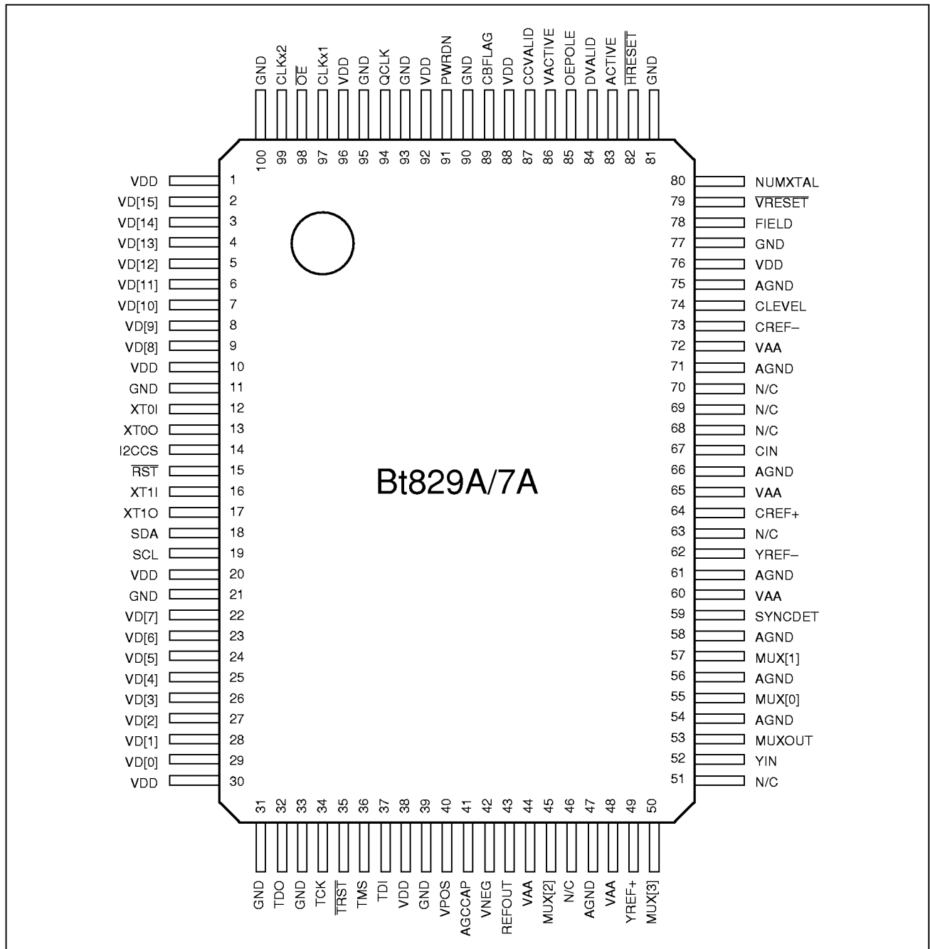
Figure 2. Bt829A/7A Pinout
