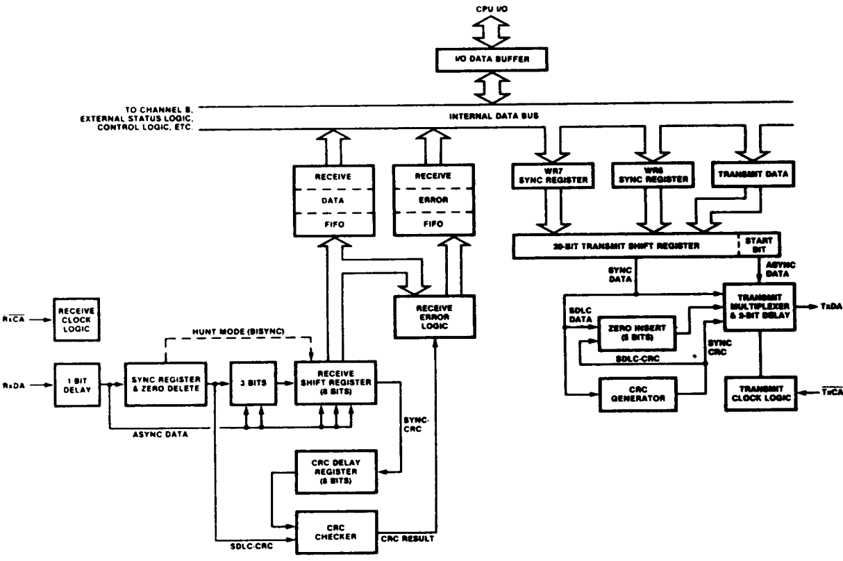
Figure 12. Transmit and Receive Data Path (Channel A)
