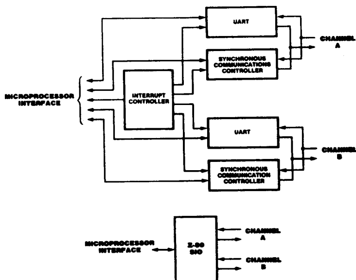
Figure 8. Conventional Devices Replaced by the Z-80 SIO
