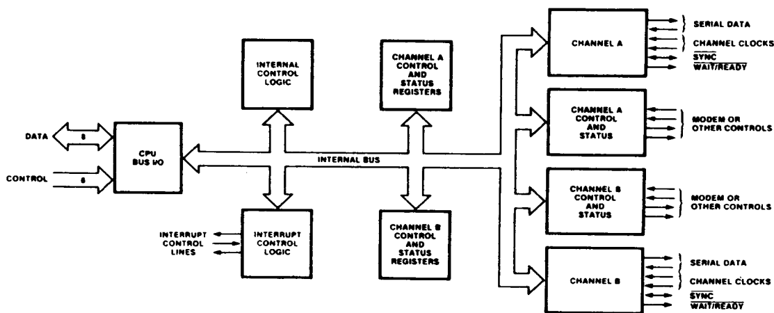
Figure 7. Block Diagram
