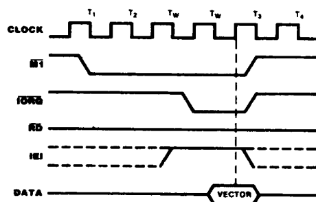
Figure 17. Interrupt Acknowledge Cycle
