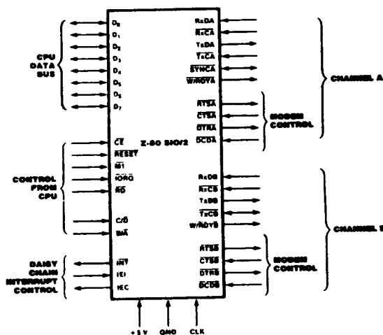
Figure 1. Z-80 SIO/2 Pin Functions
