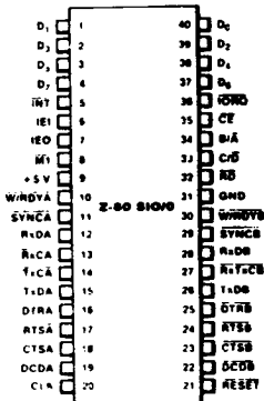
Figure 6. Z-80 SIO/0 Pin Assignments
