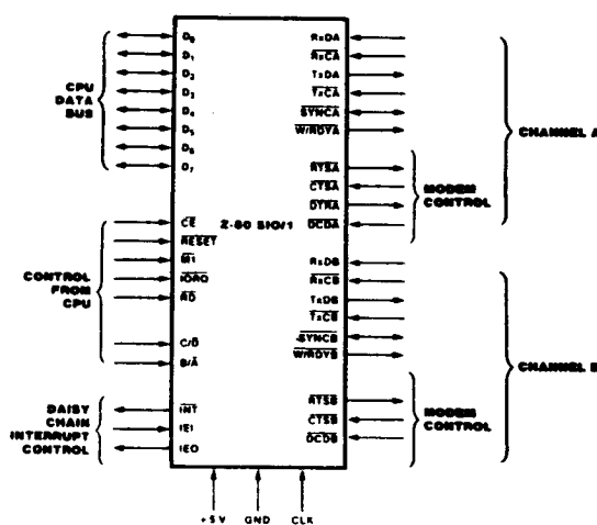
Figure 3. Z-80 SIO/1 Pin Functions
