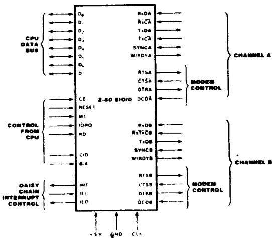
Figure 5. Z-80 SIO/0 Pin Functions
