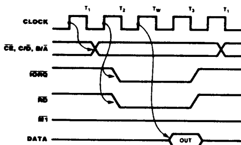
Figure 15. Read Cycle
