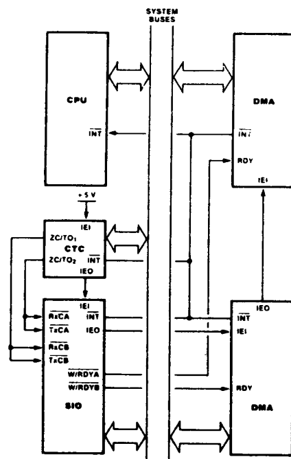
Figure 11. Typical Z-80 Environment
