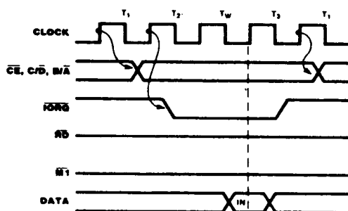
Figure 16. Write Cycle
