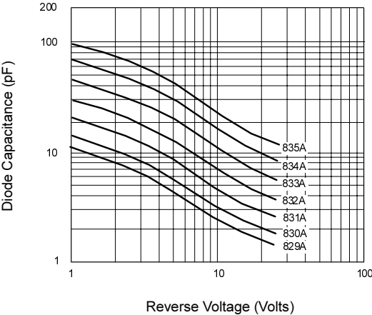
Diode Capacitance
