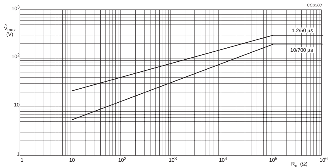
Fig.5 Maximum permissible peak pulse voltage without failing to 'open circuit' in accordance with DIN IEC 60040 (CO) 533 for type: RC31 .
