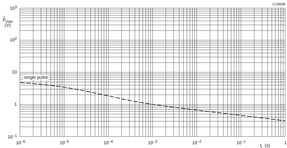
Fig.12 Pulse on a regular basis for type: RC31 ; maximum permissible peak pulse power ( \hat{P}_{max} ) as a function of pulse duration for single pulse and repetitive pulse t_p/t_i = 1000 .
