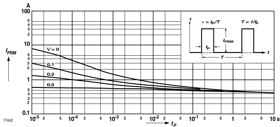
Fig. 6 Admissible Repetitive Peak Forward Current vs. Pulse Duration
