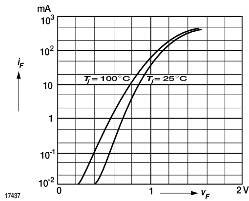
Fig. 1 Forward characteristics
