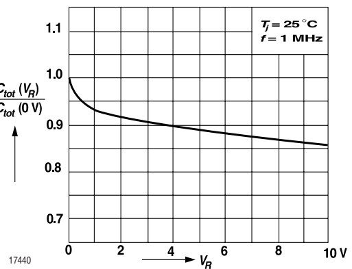
Fig. 4 Relative Capacitance vs. Reverse Voltage
