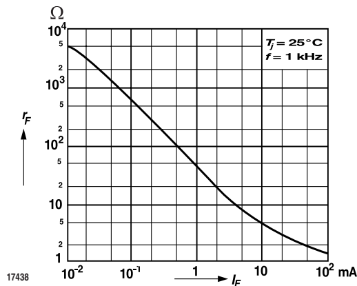
Fig. 2 Dynamic Forward Resistance vs. Forward Current
