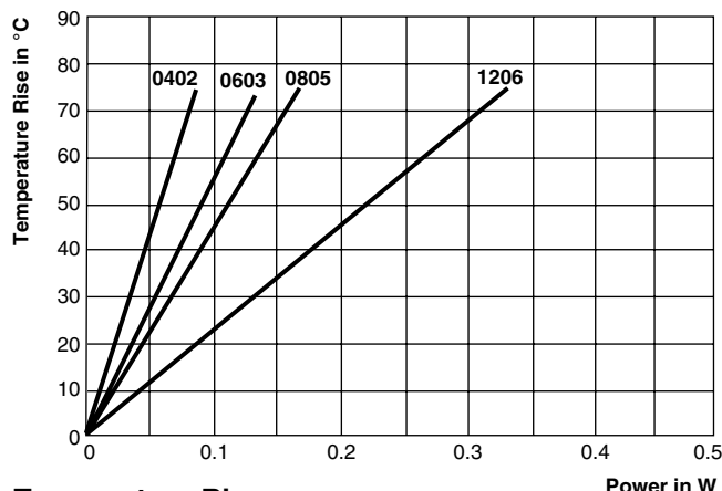
Temperature Rise
