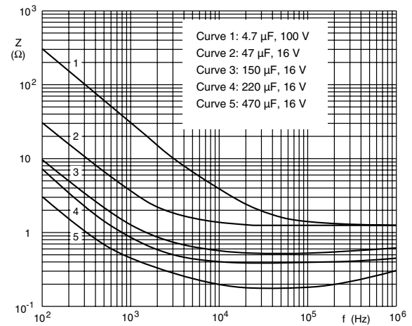
Fig.10 Typical impedance as a function of frequency
