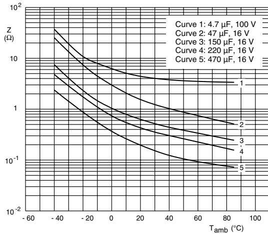
Fig.9 Typical impedance as a function of ambient temperature
