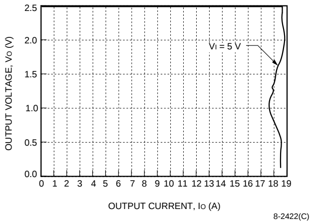
Figure 13. NH033G-L Current Limit, T_A = 25\text{ }^{\circ}\text{C}
