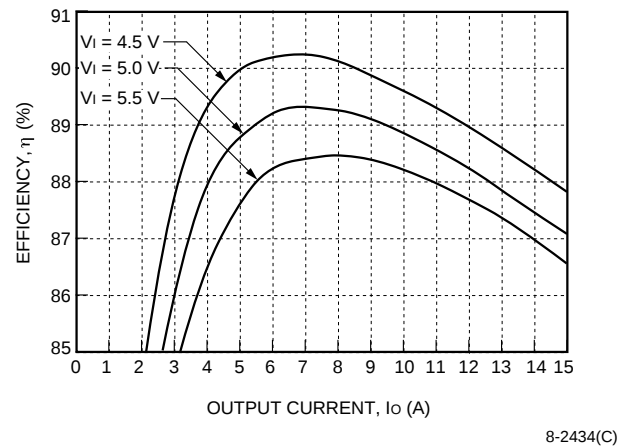
Figure 22. NH050G-L Efficiency, T_A = 25^\circ\text{C}
