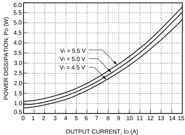
Figure 47. NH050G-L Typical Power Dissipation vs. Output Current, T_A = 25\text{ °C}
