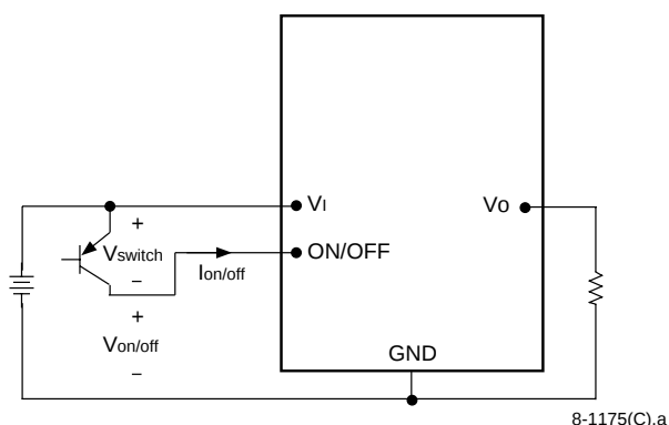
Figure 38. Remote On/Off Implementation
