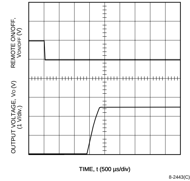
Figure 30. NH050G-L Typical Start-Up from Remote On/Off, V I = 5 V, I O = 15 A
