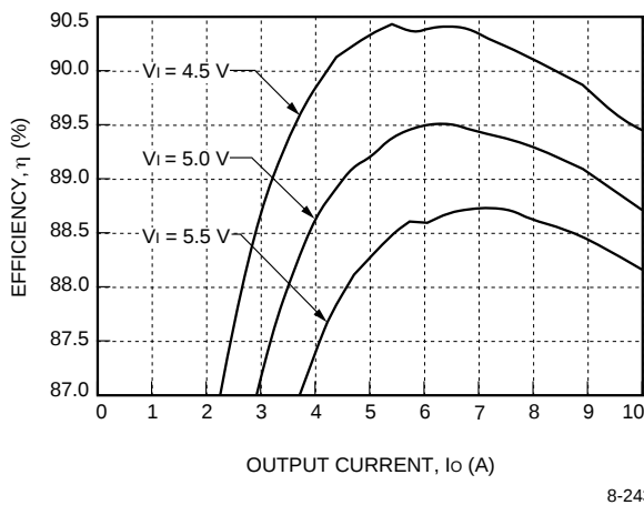
Figure 21. NH033G-L Efficiency, T_A = 25^\circ\text{C}
