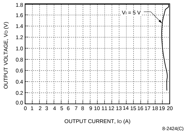
Figure 11. NH033S1R8-L Current Limit, T_A = 25\text{ }^{\circ}\text{C}
