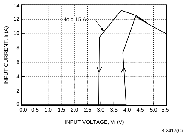
Figure 8. NH050F-L Input Characteristics, T_A = 25\text{ }^{\circ}\text{C}
