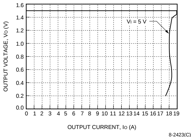
Figure 9. NH033M-L Current Limit, T_A = 25\text{ }^{\circ}\text{C}
