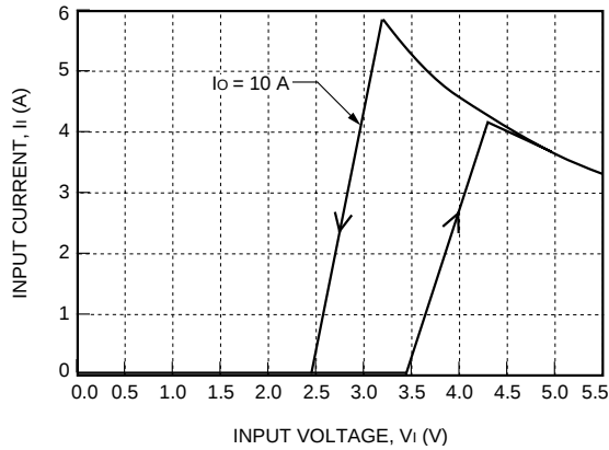
Figure 1. NH033M-L Input Characteristics, T_A = 25\text{ }^{\circ}\text{C}
