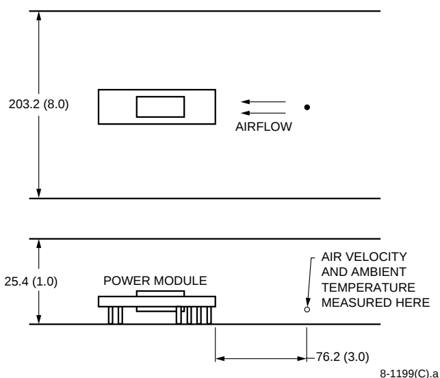
Figure 40. Thermal Test Setup
