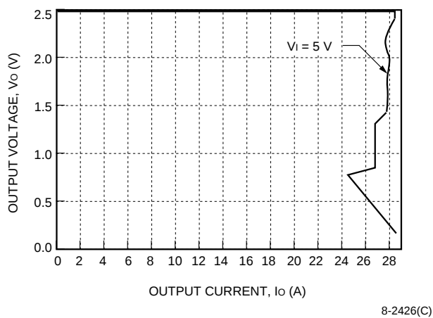
Figure 14. NH050G-L Current Limit, T_A = 25\text{ }^{\circ}\text{C}
