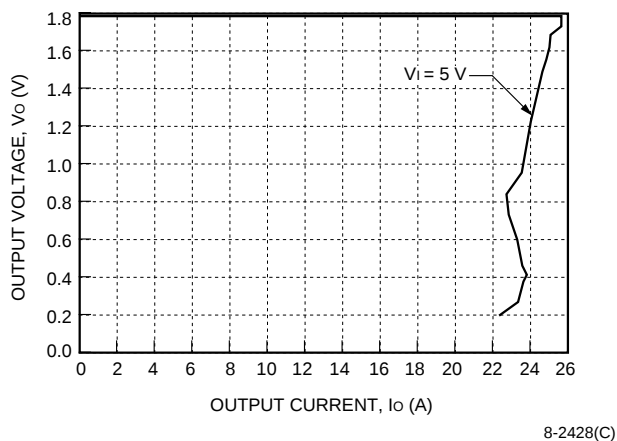
Figure 12. NH050S1R8-L Current Limit, T_A = 25\text{ }^{\circ}\text{C}
