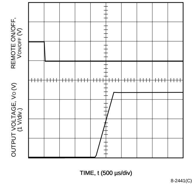
Figure 32. NH050F-L Typical Start-Up from Remote On/Off, V I = 5 V, I O = 15 A
