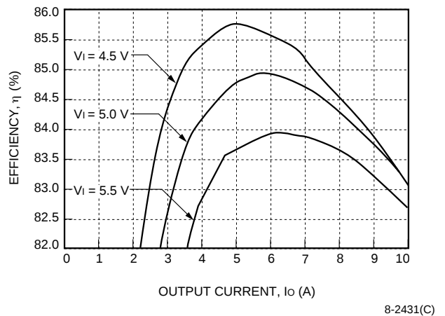
Figure 17. NH033M-L Efficiency, T_A = 25\text{ }^{\circ}\text{C}
