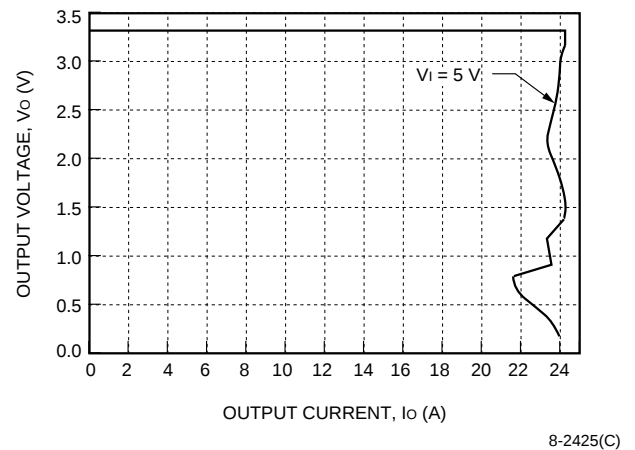
Figure 16. NH050F-L Current Limit, T_A = 25\text{ }^{\circ}\text{C}
