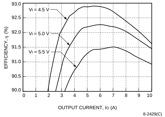
Figure 23. NH033F-L Efficiency, T_A = 25^\circ\text{C}
