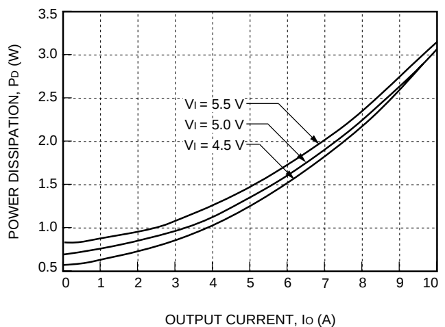
Figure 42. NH033M-L Typical Power Dissipation vs. Output Current, T_A = 25\text{ °C}
