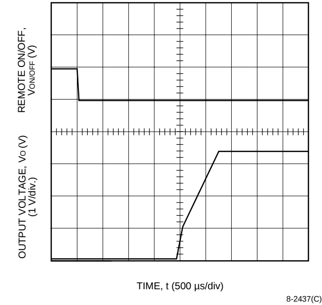
Figure 31. NH033F-L Typical Start-Up from Remote On/Off, V I = 5 V, I O = 10 A
