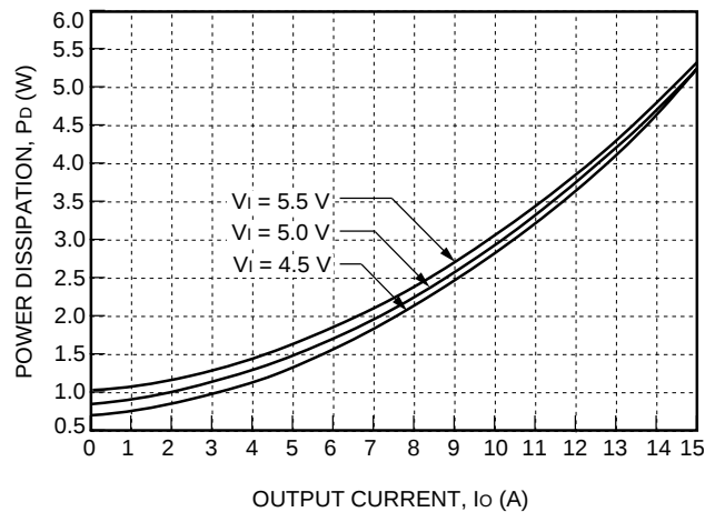
Figure 43. NH050M-L Typical Power Dissipation vs. Output Current, T_A = 25\text{ °C}
