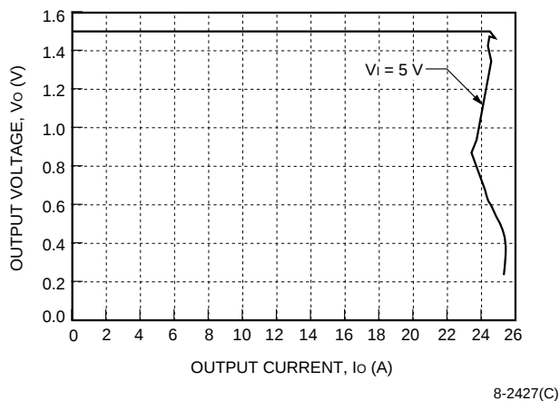
Figure 10. NH050M-L Current Limit, T_A = 25\text{ }^{\circ}\text{C}
