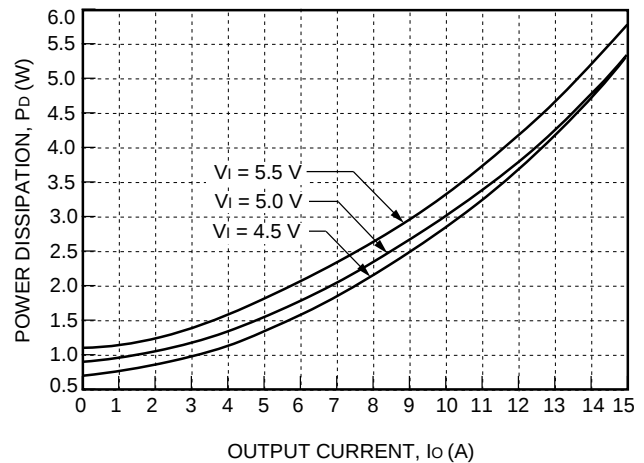
Figure 49. NH050F-L Typical Power Dissipation vs. Output Current, T_A = 25\text{ °C}
