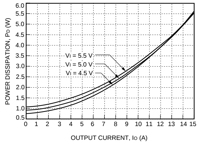
Figure 45. NH050S1R8-L Typical Power Dissipation vs. Output Current, T_A = 25\text{ °C}
