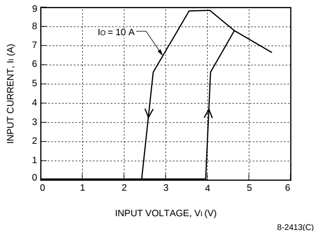
Figure 7. NH033F-L Input Characteristics, T_A = 25\text{ }^{\circ}\text{C}
