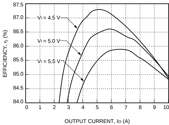
Figure 19. NH033S1R8-L Efficiency, T_A = 25^\circ\text{C}
