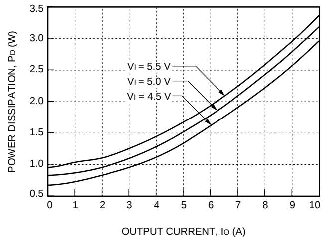
Figure 46. NH033G-L Typical Power Dissipation vs. Output Current, T_A = 25\text{ °C}
