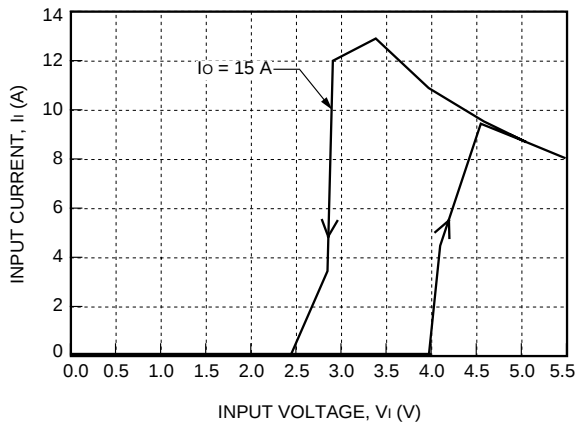
Figure 6. NH050G-L Input Characteristics, T_A = 25\text{ }^{\circ}\text{C}
