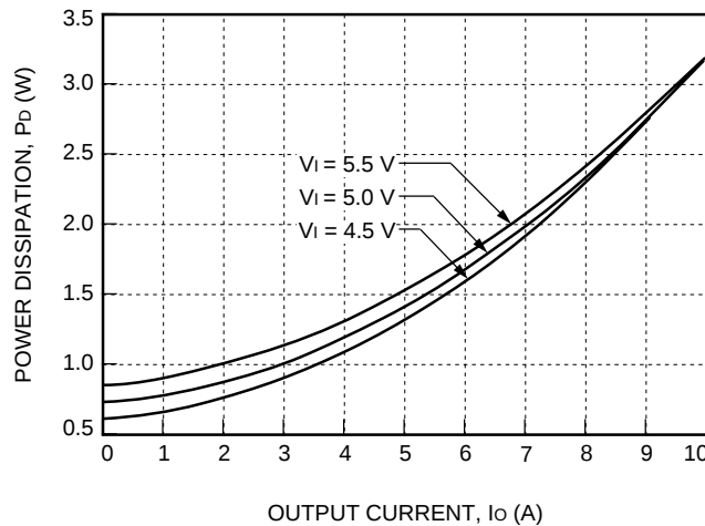
Figure 44. NH033S1R8-L Typical Power Dissipation vs. Output Current, T_A = 25\text{ °C}
