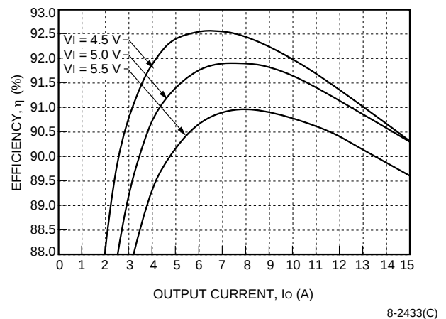
Figure 24. NH050F-L Efficiency, T_A = 25^\circ\text{C}
