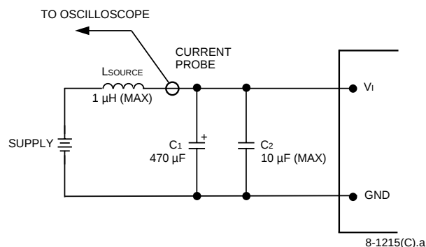
Figure 36. Setup with External Capacitor to Reduce Input Ripple Voltage
