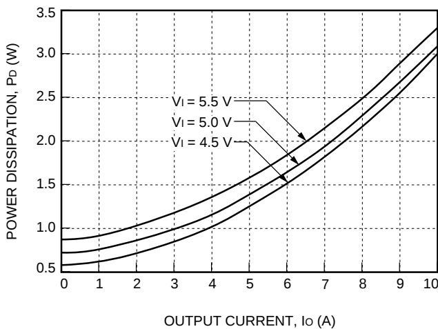
Figure 48. NH033F-L Typical Power Dissipation vs. Output Current, T_A = 25\text{ °C}
