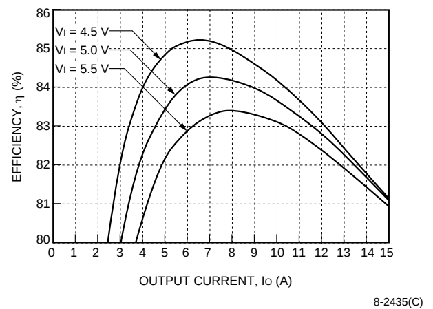
Figure 18. NH050M-L Efficiency, T_A = 25\text{ }^{\circ}\text{C}
