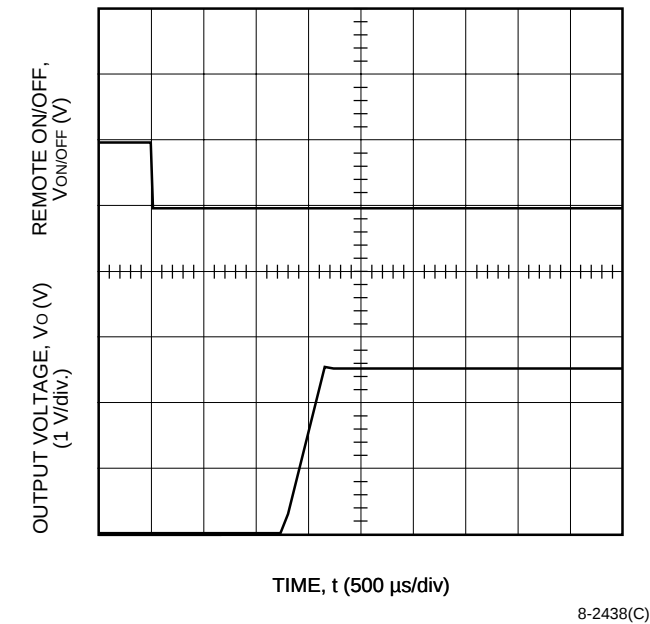
Figure 29. NH033G-L Typical Start-Up from Remote On/Off, V I = 5 V, I O = 10 A
