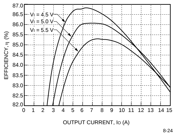
Figure 20. NH050S1R8-L Efficiency, T_A = 25^\circ\text{C}
