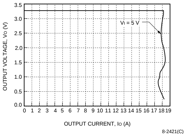
Figure 15. NH033F-L Current Limit, T_A = 25\text{ }^{\circ}\text{C}
