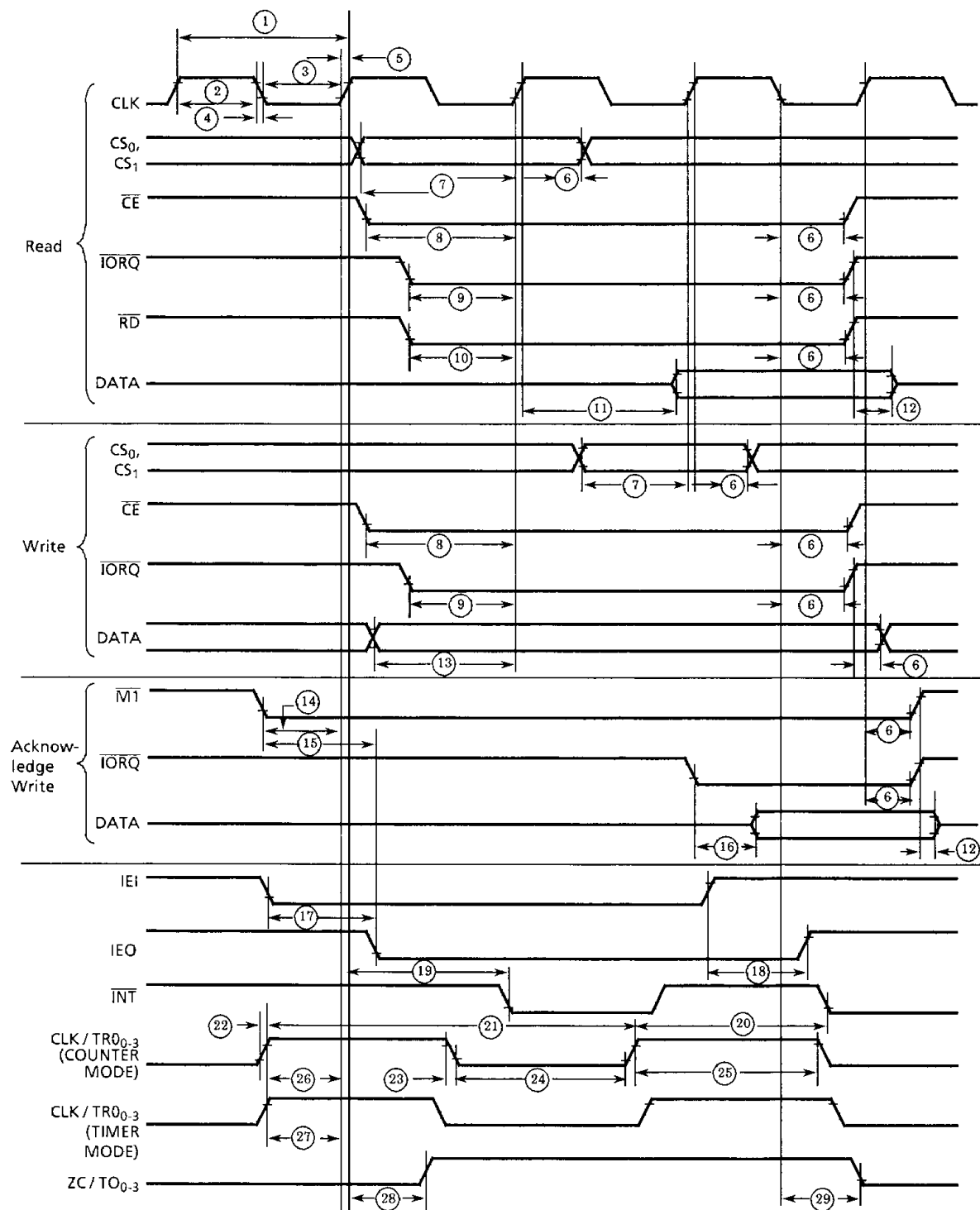
Figure 4.1 Timing Diagram
