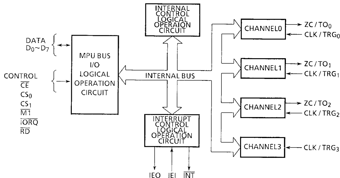
Figure 3.1 Block Diagram
