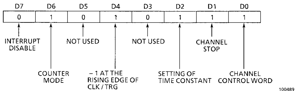
Figure 3.15 Channel Control Word Configuration
