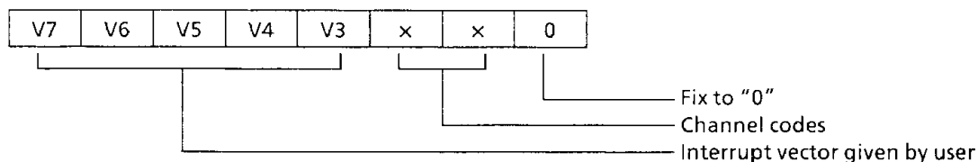
Figure 3.12 Interrupt Vector
