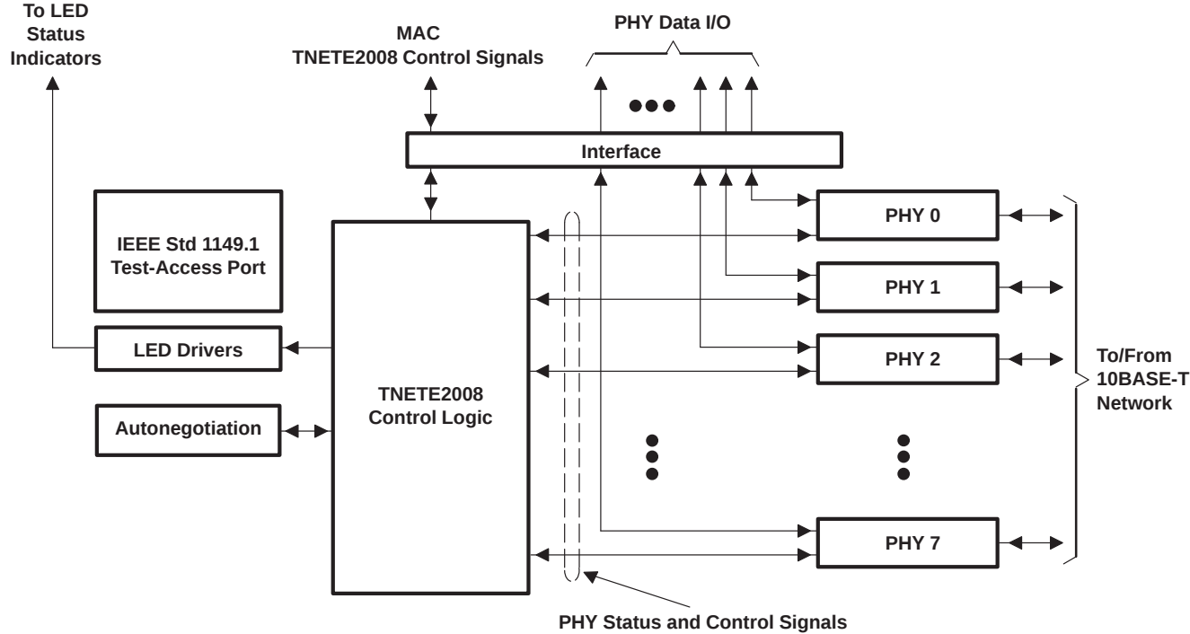
Figure 1. OctalPHY Architecture
