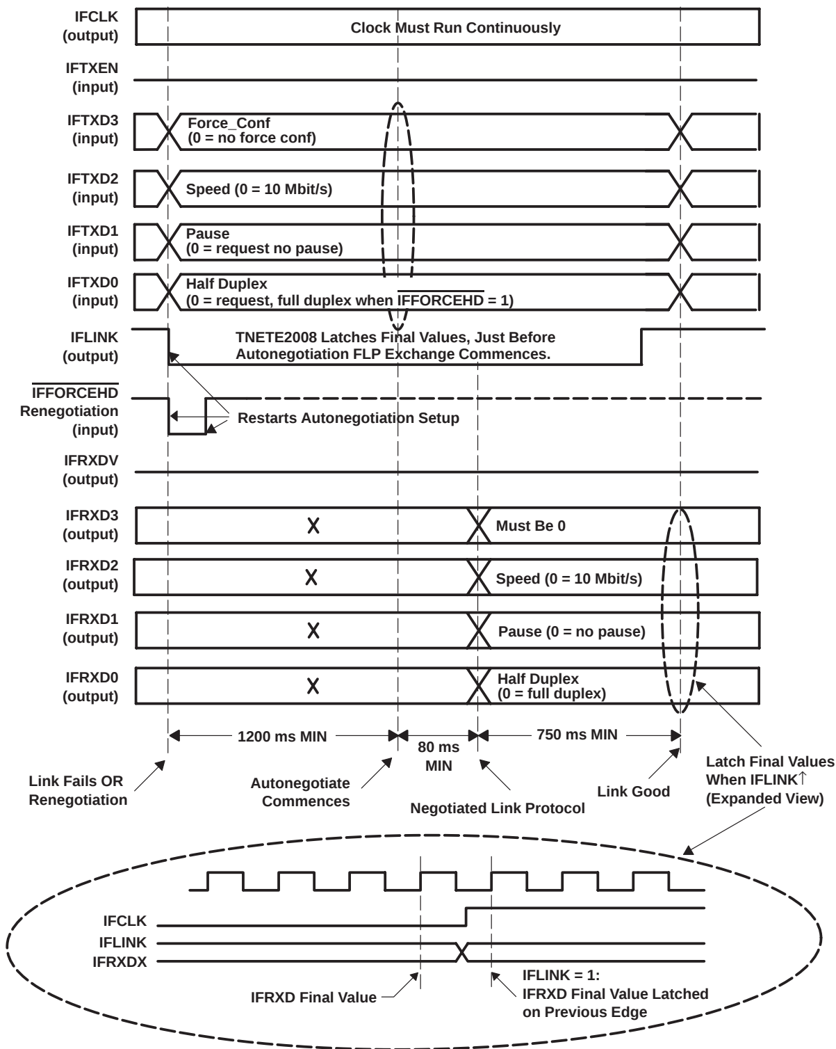
Figure 8. MAC-to-PHY, PHY-to-MAC Control Exchanges for Not Force Configuration Mode
