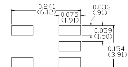
FOOTPRINT FOR PCB DESIGN
