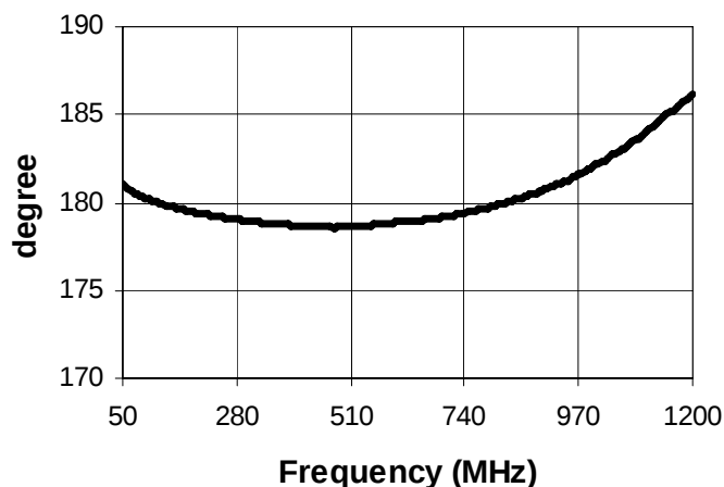
Phase Balance
