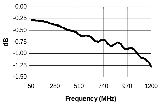
Amplitude Unbalance
