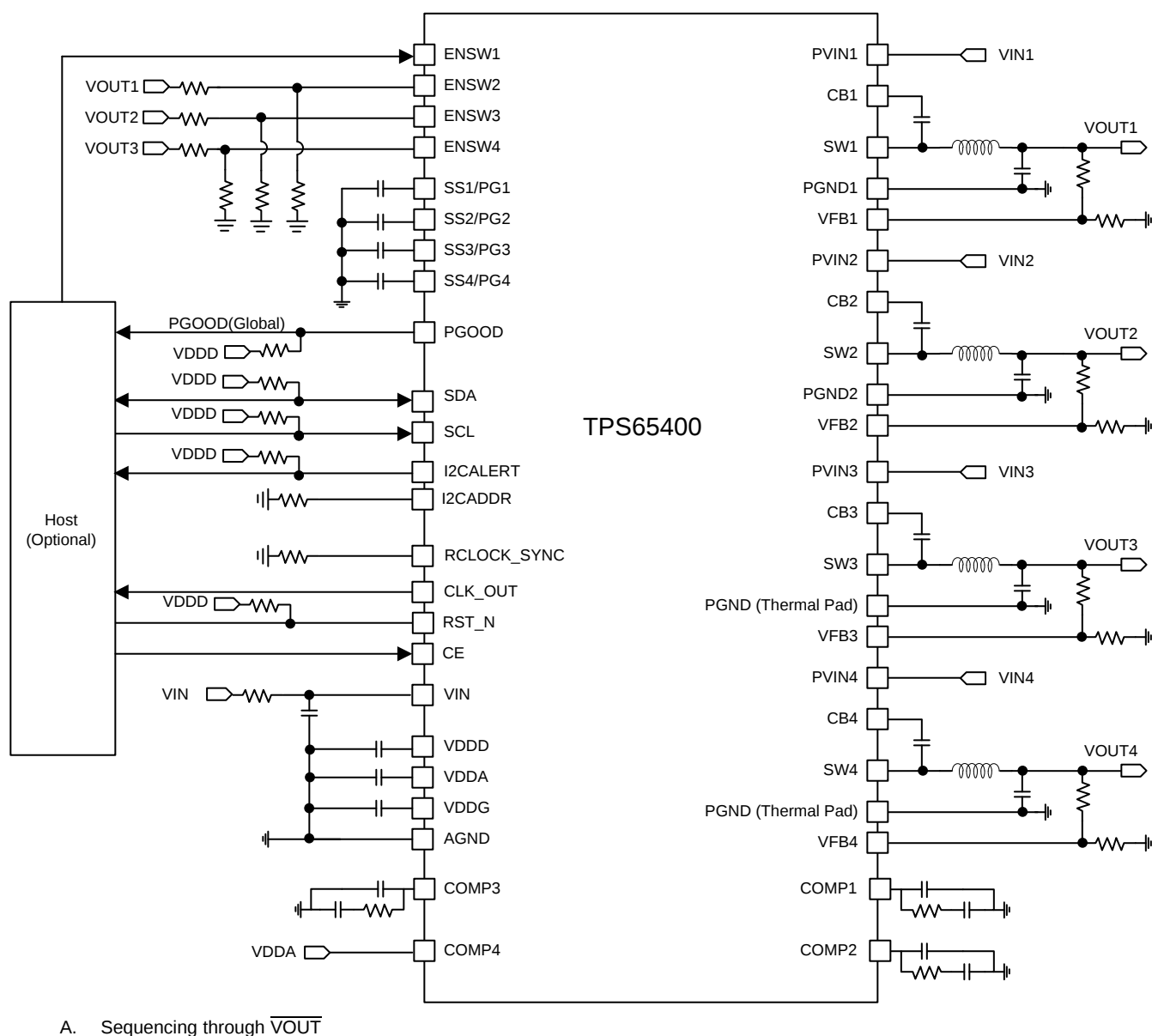
Figure 44. External Sequencing Schematic, \overline{V_{out}} > V_{EN}
