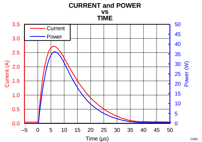
Figure 5. Surge Curve (tp = 8/20µs), Pin IO to GND
