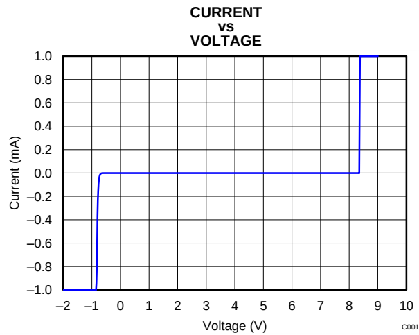
Figure 4. DC Voltage Sweep I-V Curve
