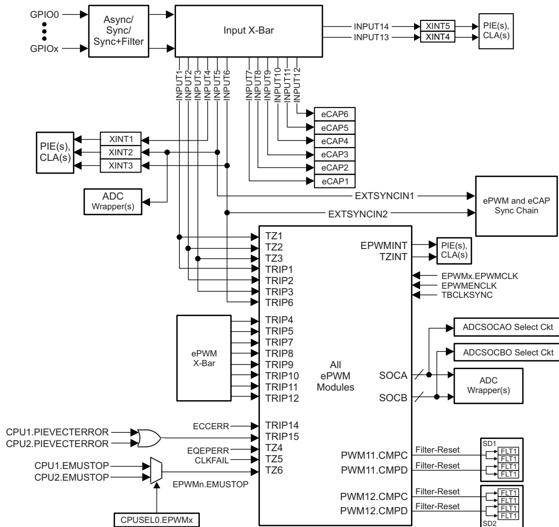
Figure 5-48. ePWM Trip Input Connectivity
