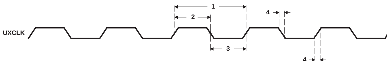
Figure 7-74. UXCLK Timing
