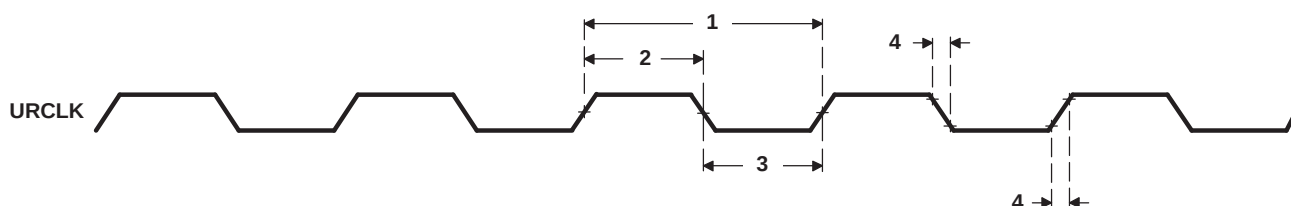
Figure 7-75. URCLK Timing
