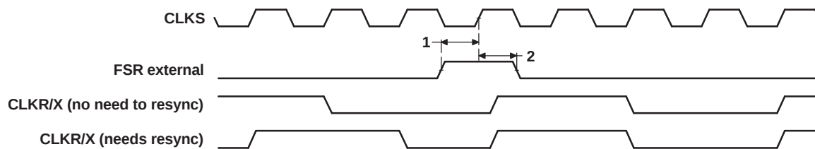
Figure 7-53. FSR Timing When GSYNC = 1
