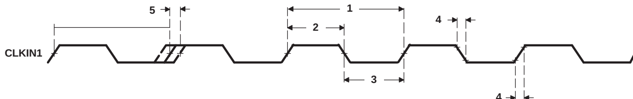
Figure 7-21. CLKIN1 Timing
