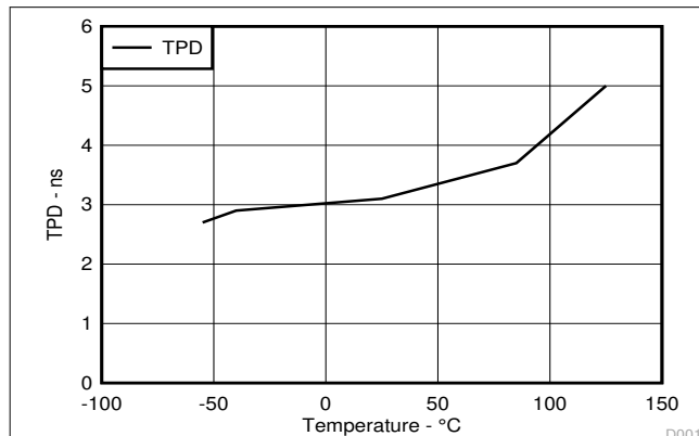
Figure 5-1. TPD Across Temperature at 3.3\text{V } V_{CC}
