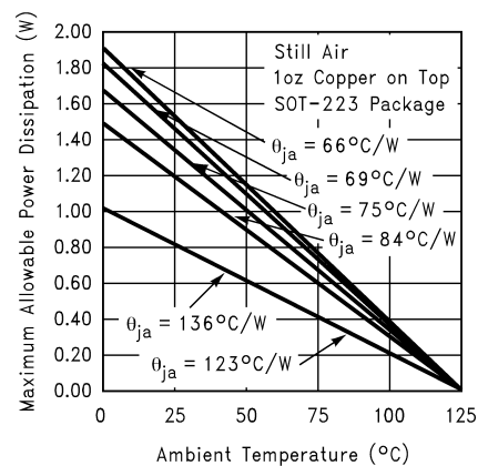
Figure 27. Maximum Allowable Power Dissipation vs. Ambient Temperature for SOT-223
