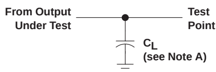
LOAD CIRCUIT FOR t_r and t_f
