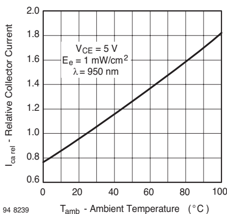
Figure 3. Relative Collector Current vs. Ambient Temperature
