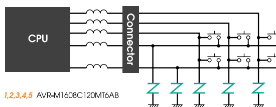
for PDA Application Circuit : Push Button
