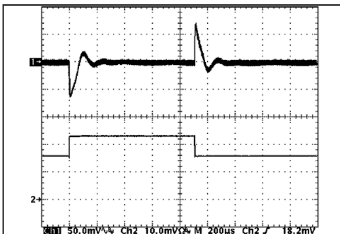
Figure 18: Output voltage response for 2.5V unit to step-change in load current (50-75-50% of I out max; di/dt=5A/µs). Load cap: 470µF, 25mΩ ESR tantalum and 1µF ceramic. Ch 1: V out (50mV/div), Ch 2: I out (5A/div).
