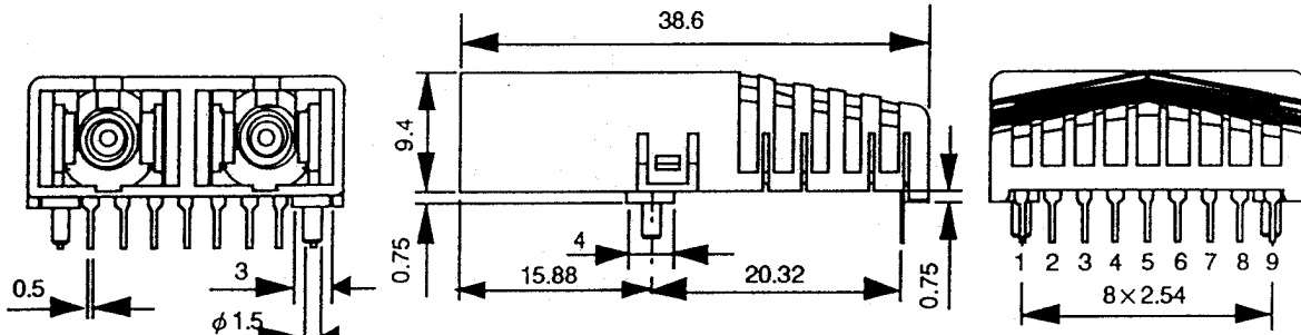
Figure 4 External View
