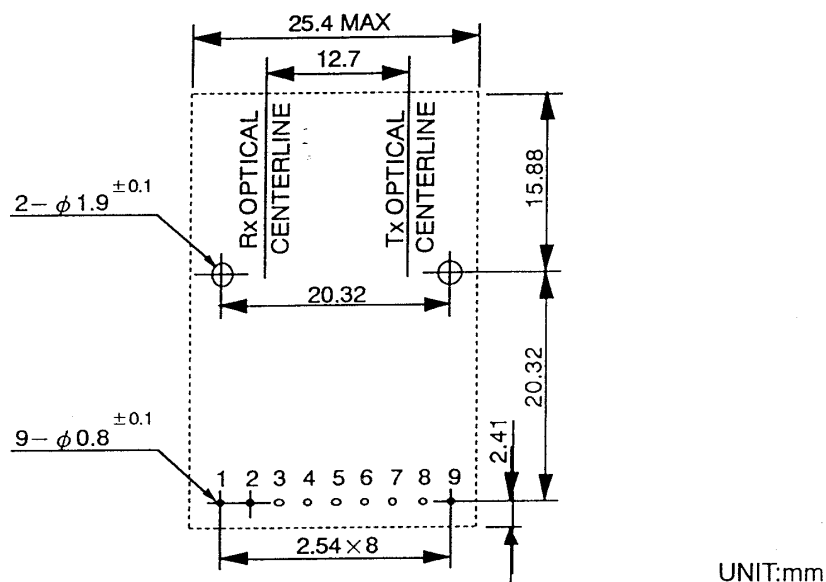
Figure 5 Footprint
