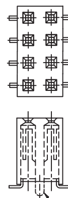
Two Row SMT, With guide post(P)
