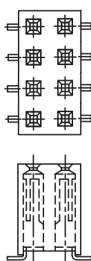
Two Row SMT, Without guide post(S)
