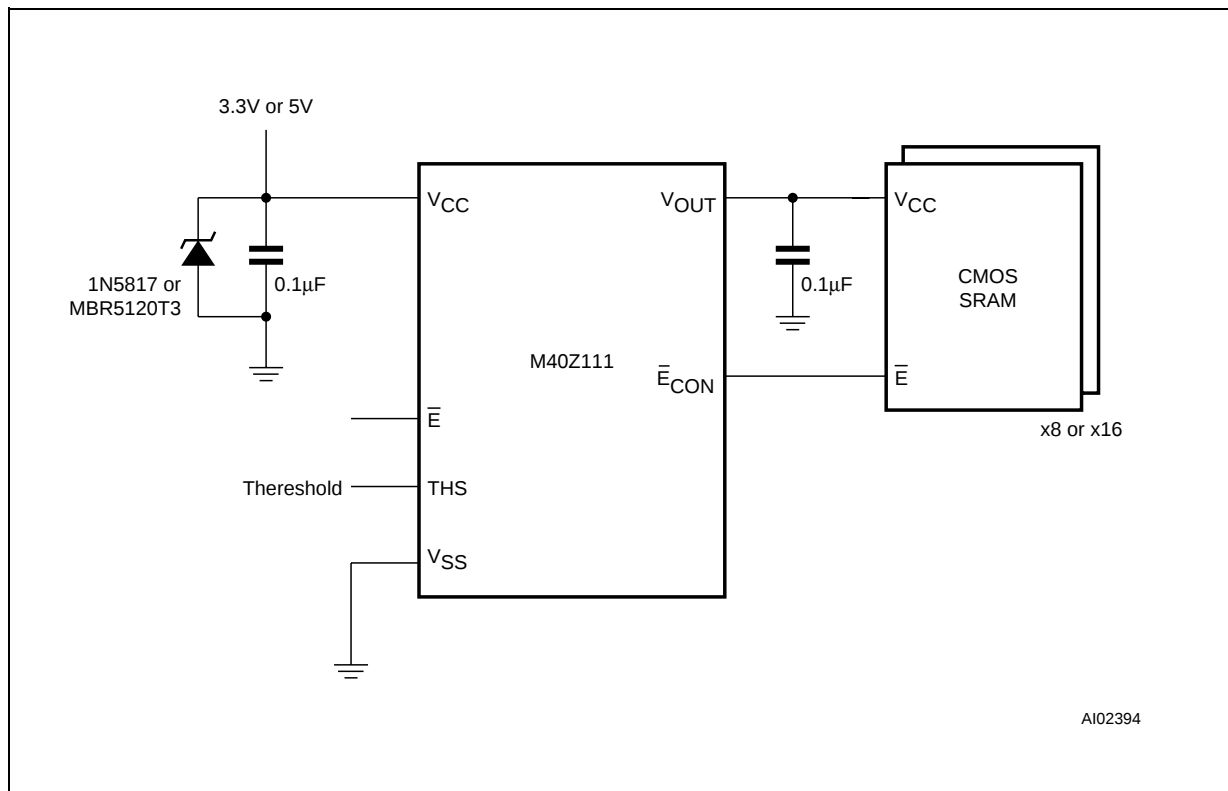
Figure 3. Hardware Hookup
