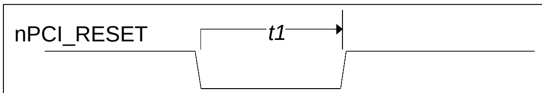
FIGURE 9C - RESET TIMING
