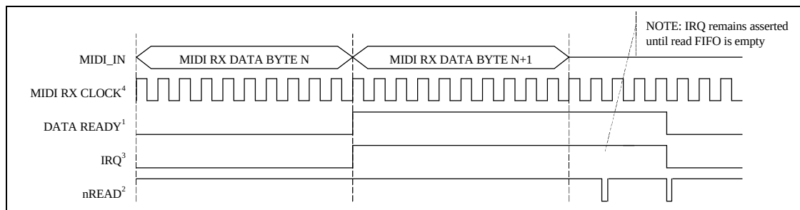
FIGURE 3 - MPU-401 INTERRUPT
