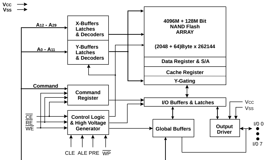
Figure 1-1. K9XXG08XXM (X8) Functional Block Diagram
