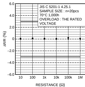
Fig.8 Endurance at 70^\circ\text{C}
