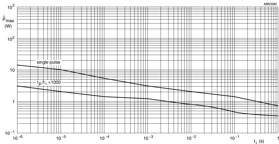
Fig.6 Pulse on a regular basis for type: RC01 ; maximum permissible peak pulse power ( \hat{P}_{max} ) as a function of pulse duration for single pulse and repetitive pulse t_p/t_i = 1000 .
