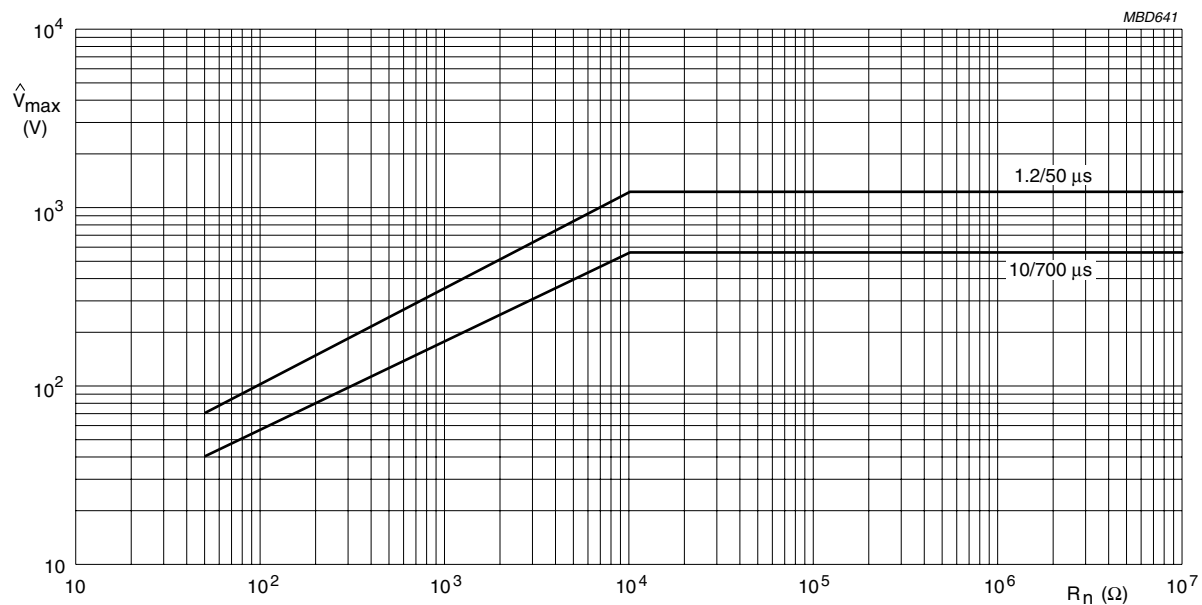
Fig.2 Maximum permissible peak pulse voltage without failing to 'open circuit' in accordance with DIN IEC 60040 (CO) 533 for type: RC01 .
