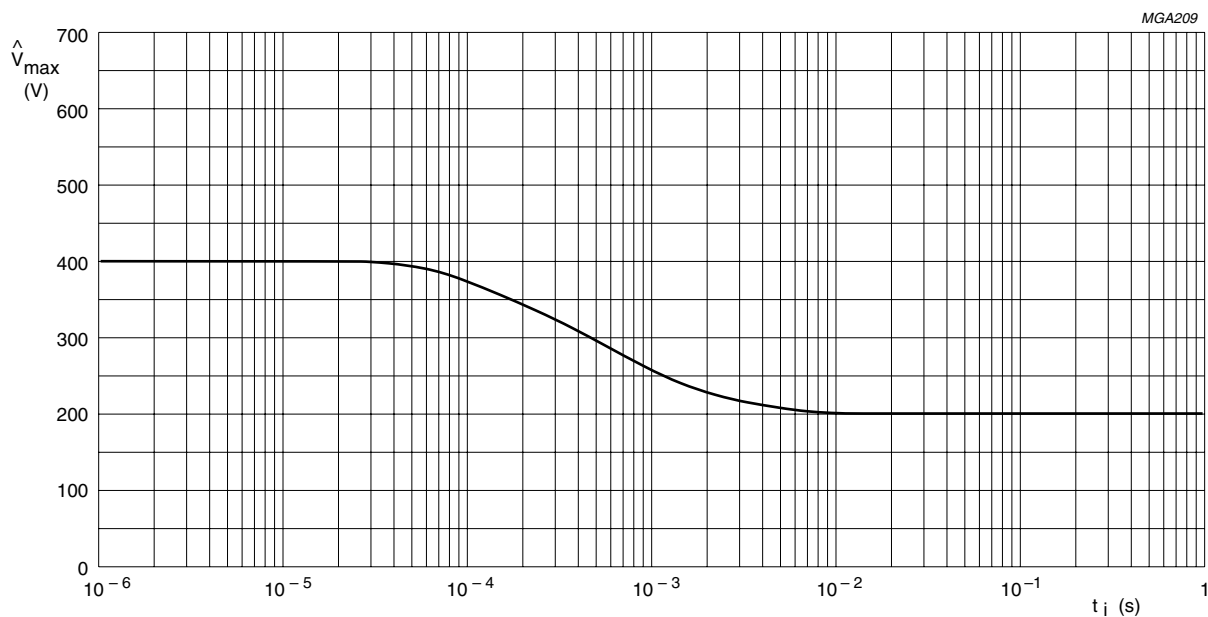
Fig.7 Pulse on a regular basis for type: RC01 ; maximum permissible peak pulse voltage ( \hat{V}_{max} ) as a function of pulse duration.
