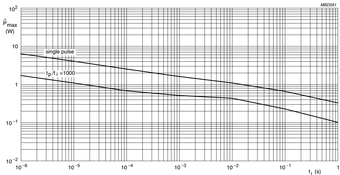
Fig.10 Pulse on a regular basis for type: RC21 ; maximum permissible peak pulse power ( \hat{P}_{max} ) as a function of pulse duration for single pulse and repetitive pulse t_p/t_i = 1000 .
