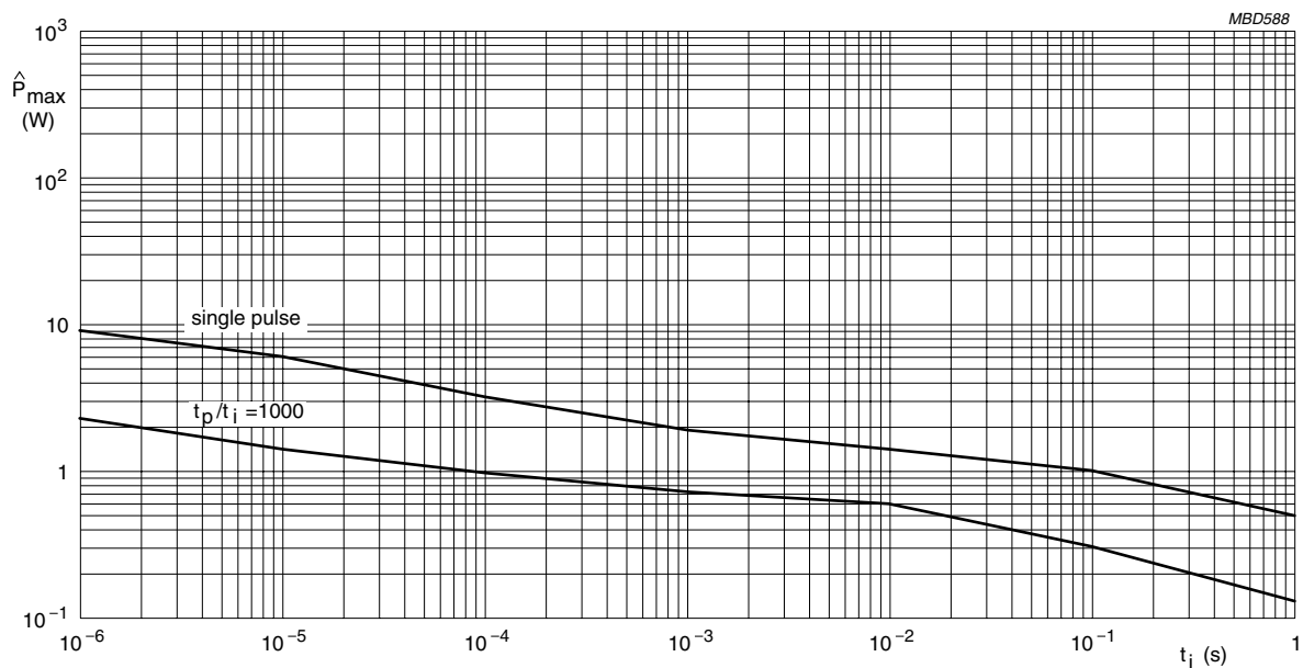
Fig.8 Pulse on a regular basis for type: RC11 ; maximum permissible peak pulse power ( \hat{P}_{max} ) as a function of pulse duration for single pulse and repetitive pulse t_p/t_i = 1000 .
