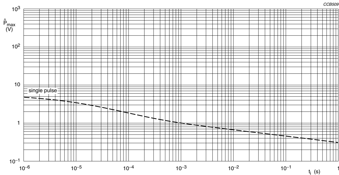
Fig.12 Pulse on a regular basis for type: RC31 ; maximum permissible peak pulse power ( \hat{P}_{max} ) as a function of pulse duration single pulse and repetitive pulse t_p/t_i = 1000 .
