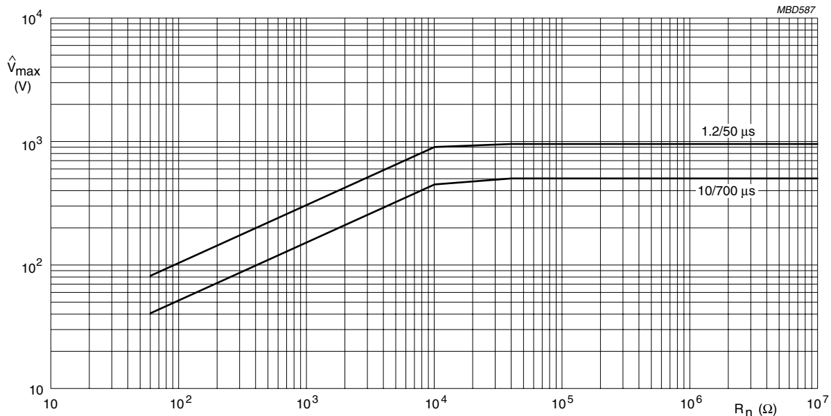
Fig.3 Maximum permissible peak pulse voltage without failing to 'open circuit' in accordance with DIN IEC 60040 (CO) 533 for type: RC11 .
