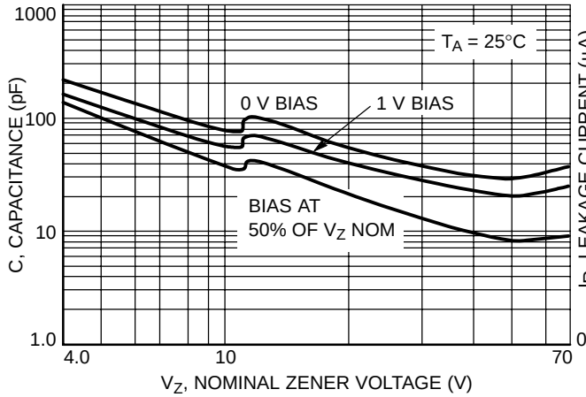
Figure 3. Typical Capacitance
