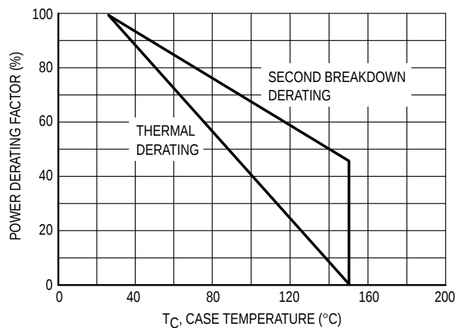
Figure 16. Power Derating
