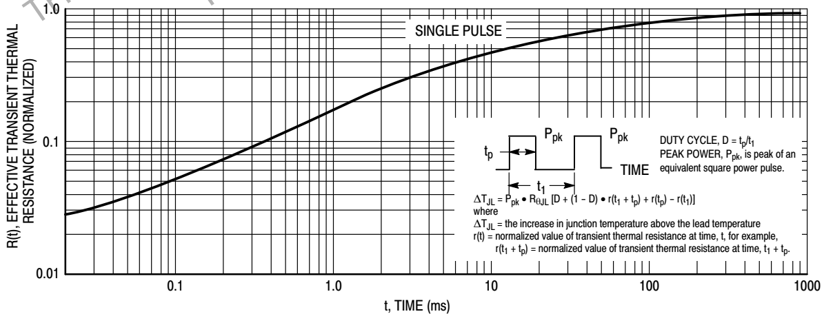
Figure 10. Thermal Response
