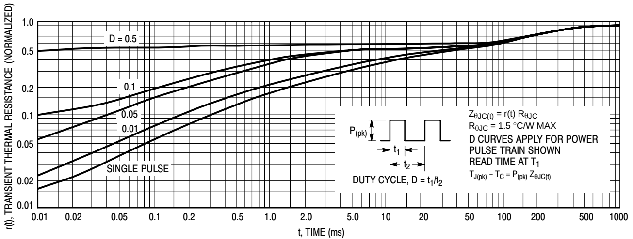
Figure 6. Thermal Response
