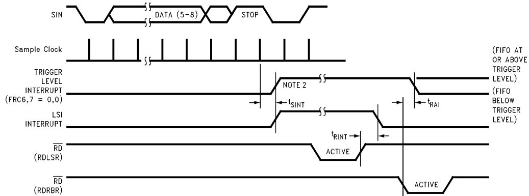
FIGURE 9-6a. Receiver Timing
