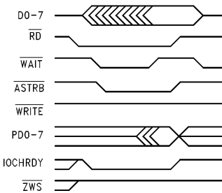
FIGURE 7-5. EPP 1.9 Address Read
