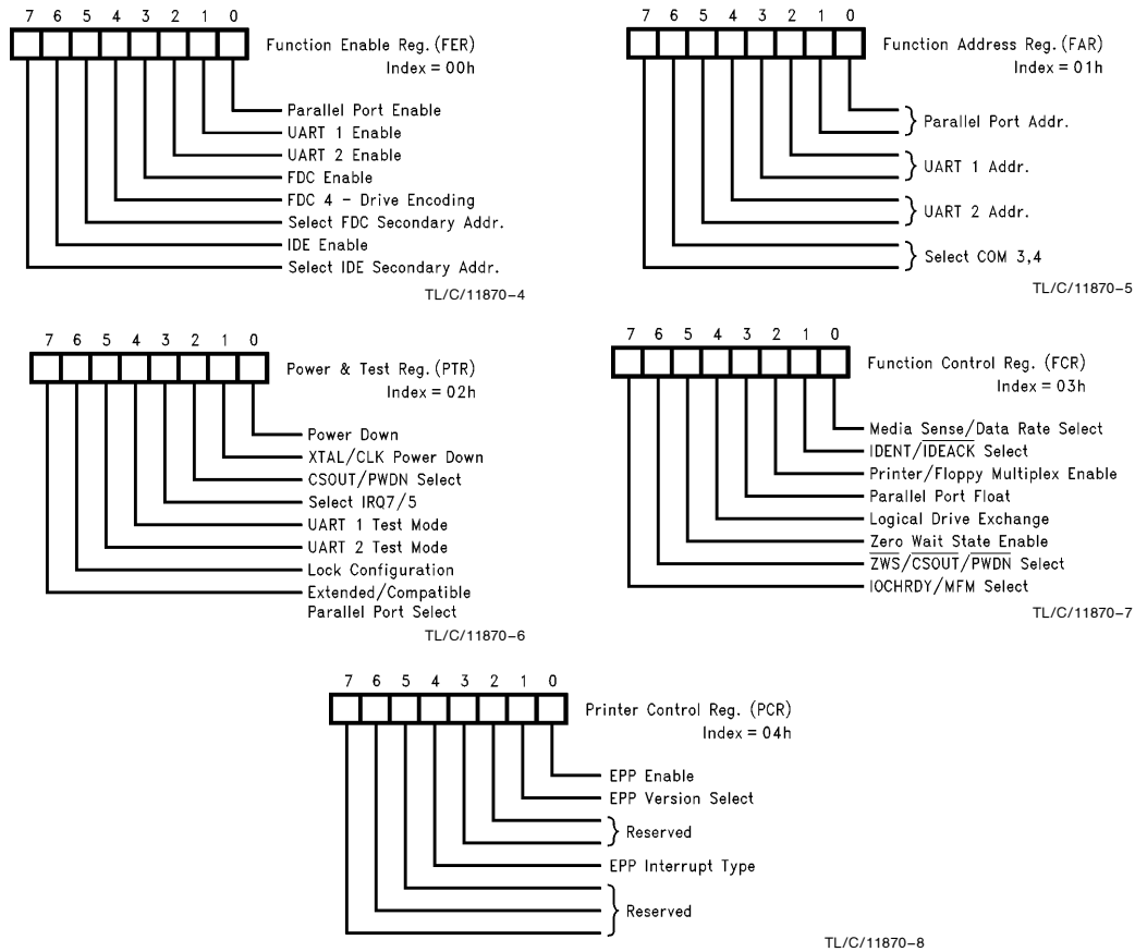
FIGURE 2-1. PC87322VF Configuration Registers
