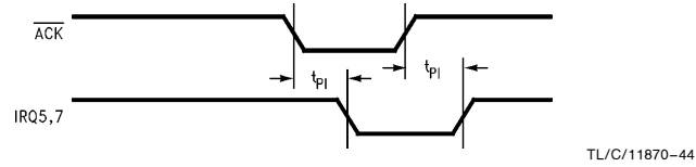
FIGURE 9-14. Parallel Port Interrupt Timing (Compatible Mode)
