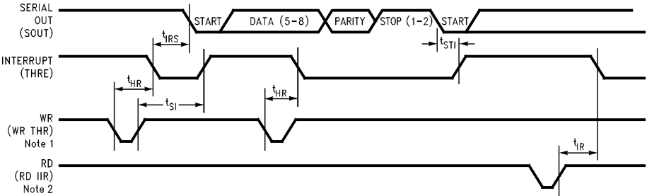
FIGURE 9-5. Transmitter Timing
