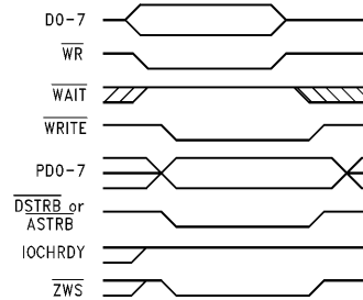
FIGURE 7-3. EPP Write with ZWS
