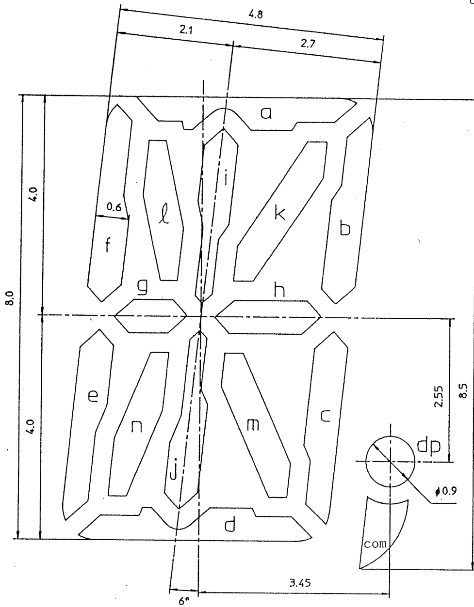
Pin Assignment
