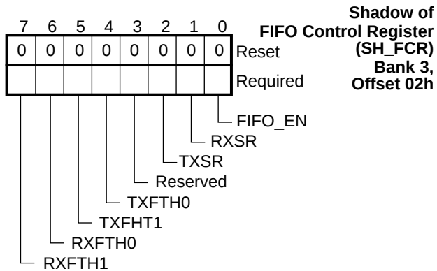
FIGURE 7-30. SH_FCR Register Bitmap
