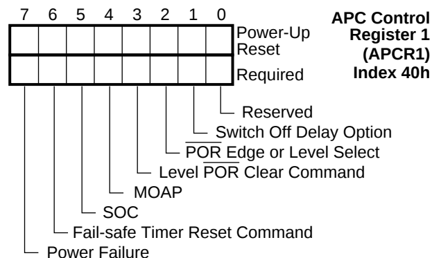
FIGURE 4-11. APCR1 Register Bitmap
