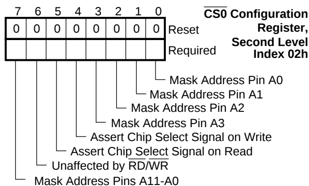
FIGURE 2-14. \overline{\text{CS0}} Configuration Register Bitmap
