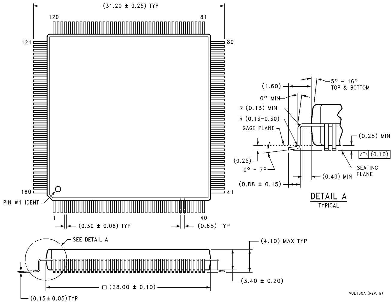
PlasticQuad Flatpack (PQFP), EIAJ Order Number PC87307VUL/PC97307VUL NS Package Number VUL160A
