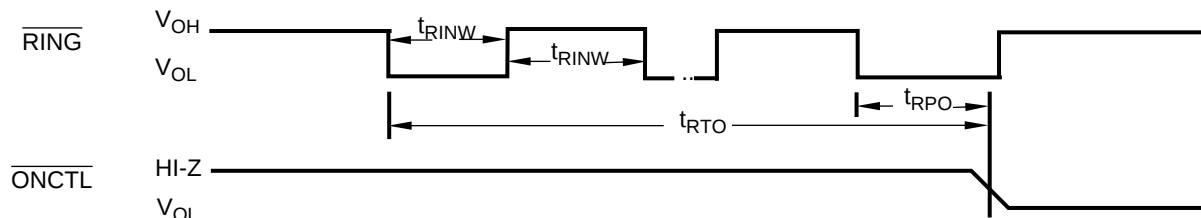
FIGURE 13-33. \overline{\text{RING}} Trigger and \overline{\text{ONCTL}} Timing
