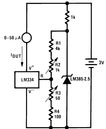
0°F–50°F Thermomemter
