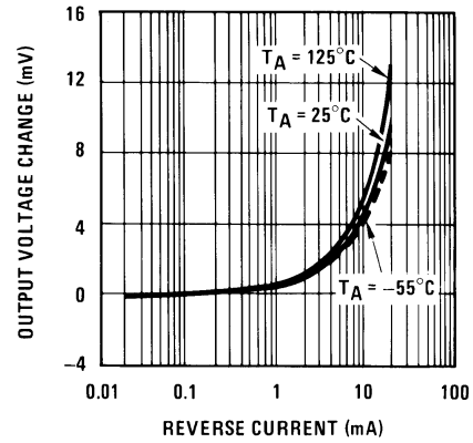
Reverse Characteristics
