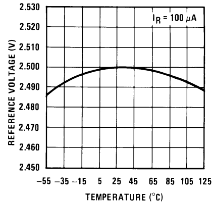
Temperature Drift
