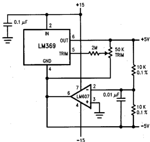
\pm 5V Reference
