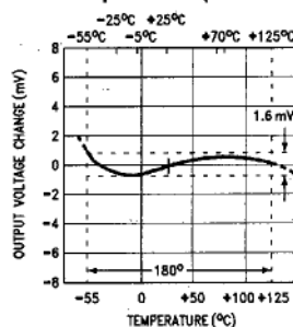
LM169 Temperature Coefficient Specified Temperatures (see Note 6)
