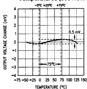
LM369 Temperature Coefficient Specified Temperatures (see Note 6)
