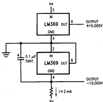
\pm 10V Reference
