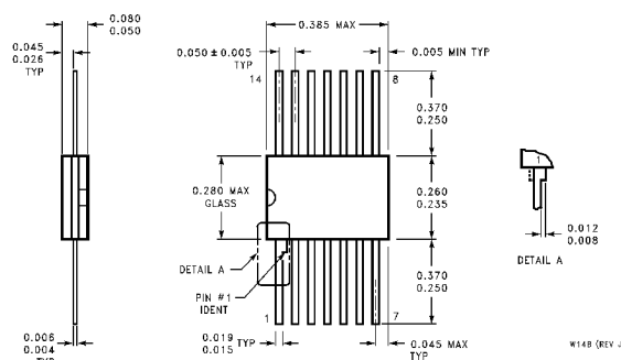
14-Lead Ceramic Flat Package (W) Order Number DM54S32W Package Number W14B
