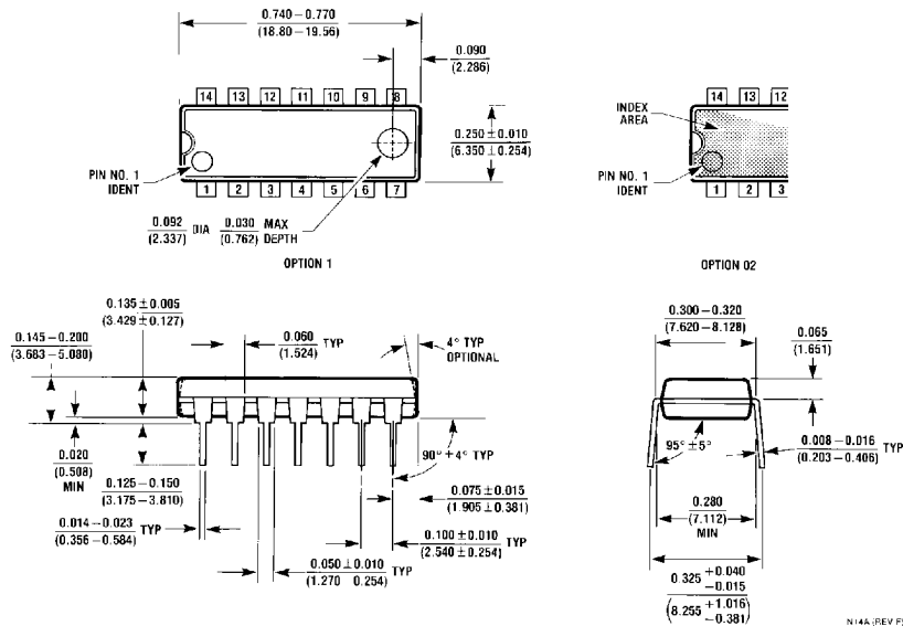
14-Lead Molded Dual-In-Line Package (N) Order Number DM74S32N Package Number N14A
