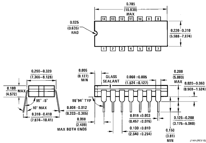
14-Lead Ceramic Dual-In-Line Package (J) Order Number DM54S32J Package Number J14A
