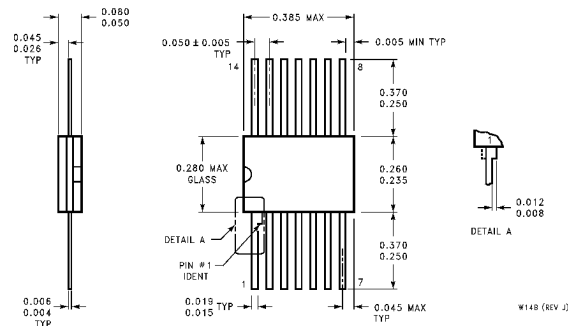
14-Lead Ceramic Flat Package (W) Order Number DM74LS86W Package Number W14B
