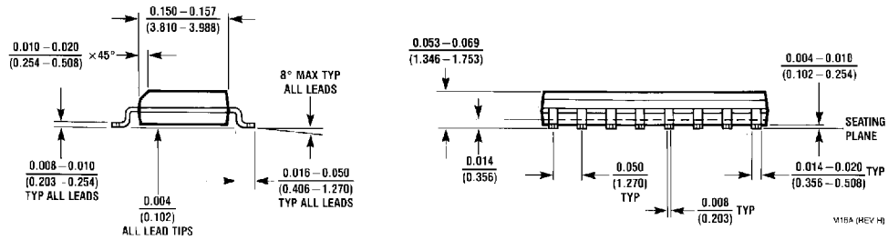
16-Lead Small Outline Molded Package (M) Order Number DM74LS75M NS Package Number M16A
