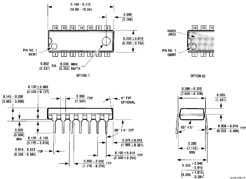
14-Lead Molded Dual-In-Line Package (N) Order Number DM74LS27N NS Package Number N14A
