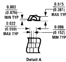
Ceramic Leadless Chip Carrier Package (E) Order Number DM54LS27E NS Package Number E20A
