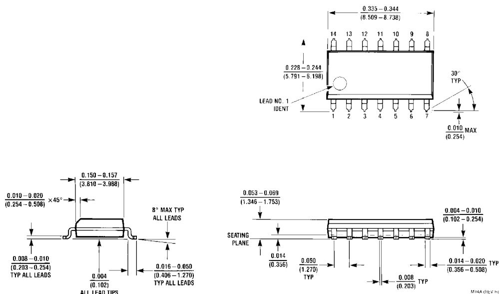
14-Lead Small Outline Molded Package (M) Order Number DM74LS27M NS Package Number M14A
