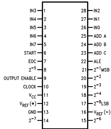
Dual-In-Line Package
