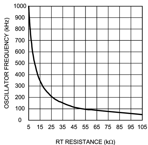
Oscillator Frequency vs RT Resistance
