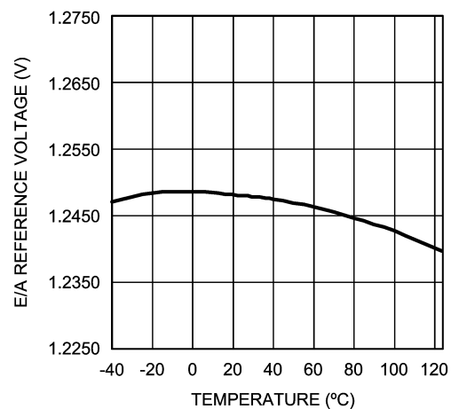
Error Amplifier Reference Voltage vs Temperature
