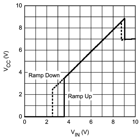
V_{CC} vs V_{IN} R_L = 7\text{k}\Omega
