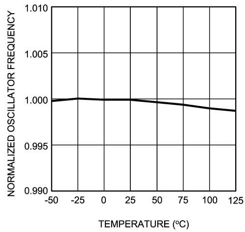
Oscillator Frequency vs Temperature F_{OSC} = 200\text{kHz}
