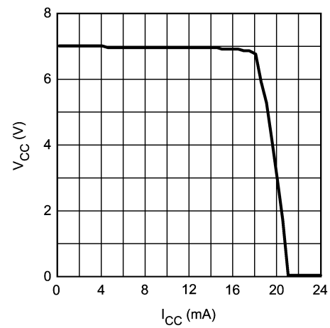
V_{CC} vs I_{CC} V_{IN} = 12\text{V}
