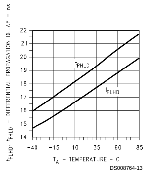
Differential Propagation Delay vs Temperature
