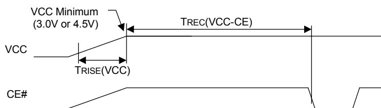
Figure 9: Reset Timing – DIP Package
