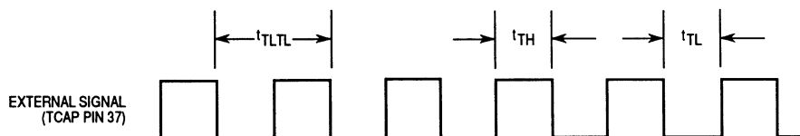
Figure 8-6. Timer Relationships
