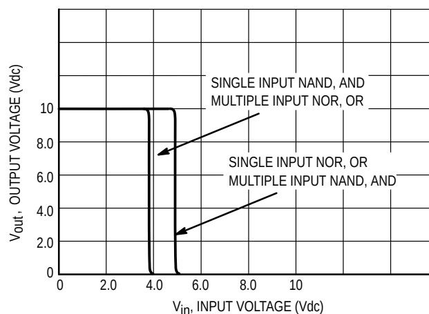
Figure 9. V_{DD} = 10 Vdc
