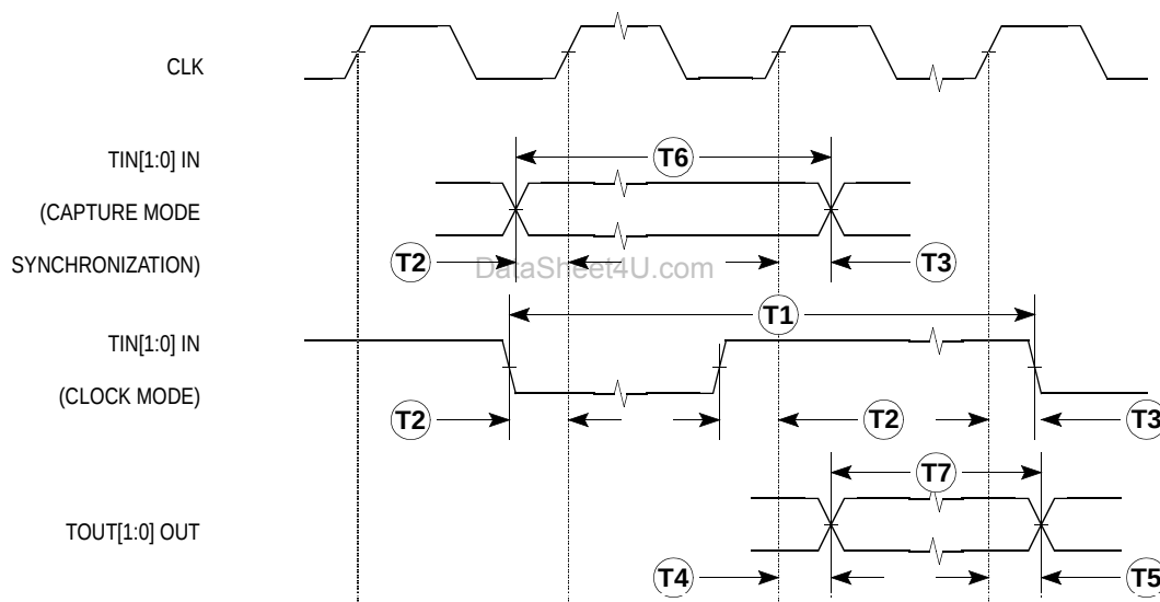
Figure 17-11. Timer Timing
