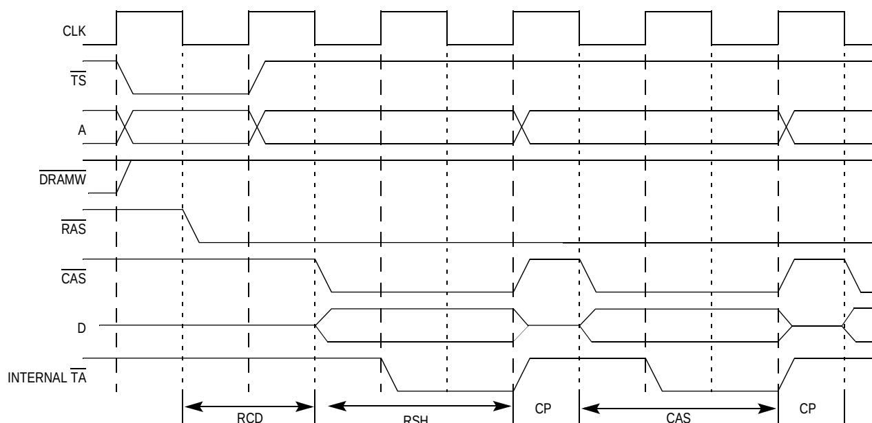
Figure 11-18. Fast Page Mode or Burst Page Mode DRAM Transfer Timing
