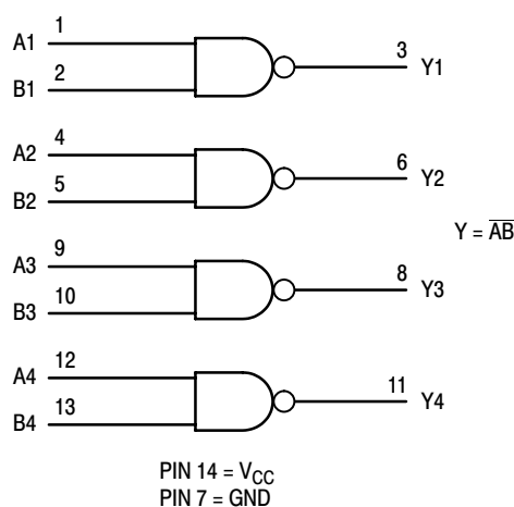
Figure 1. Logic Diagram
